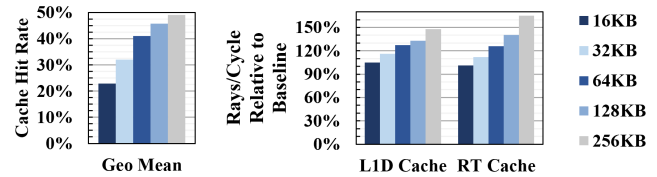
Figure 16: Cache hit rates (left) and speedup (right) for varying cache configurations.
