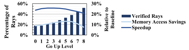
Figure 14: Increased verified rate versus decreased memory access savings for different Go Up Levels.
