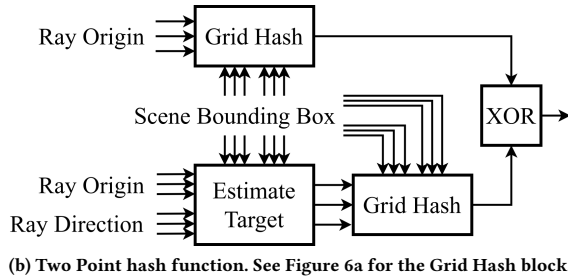
Figure 6: Hash functions
